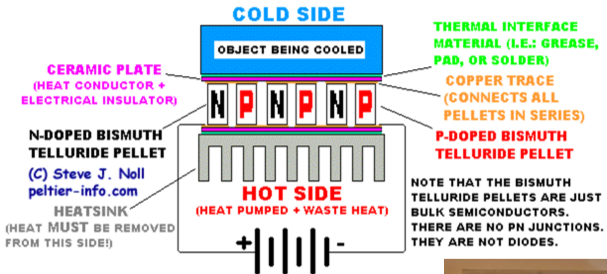
Illustration 1: Peltier Effect ThermoElectric Device
